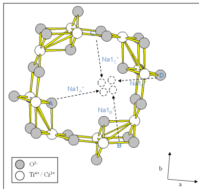
Fig. 3. Hollandite model projected slightly off the c-axis to give a clearer view of the 3-dimensional structure. When \text{Ti}_A^{4+} is replaced by \text{Cr}^{3+} , the preferable location for the \text{Na1}_A^+ ions is shown by the arrow, a similar situation is found for \text{Na1}_B^+ , \text{Na1}_C^+ and \text{Na1}_D^+ .
