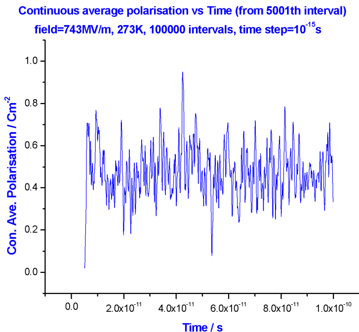
Fig. 8. Continuous average for the polarisation with an applied field of 743MV/m as a function of time.
