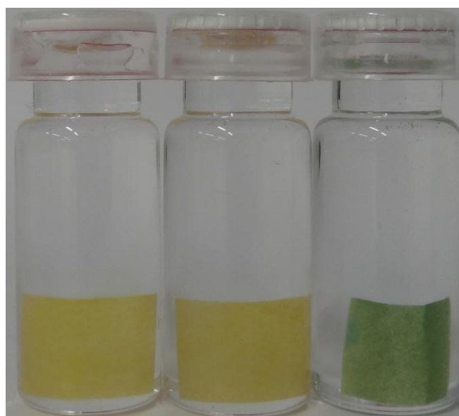
Figure 7. Samples of Ethaline (left) Glyceline (middle) and Reline (right) with 20 wt% water and each containing a sample of universal indicator paper.
