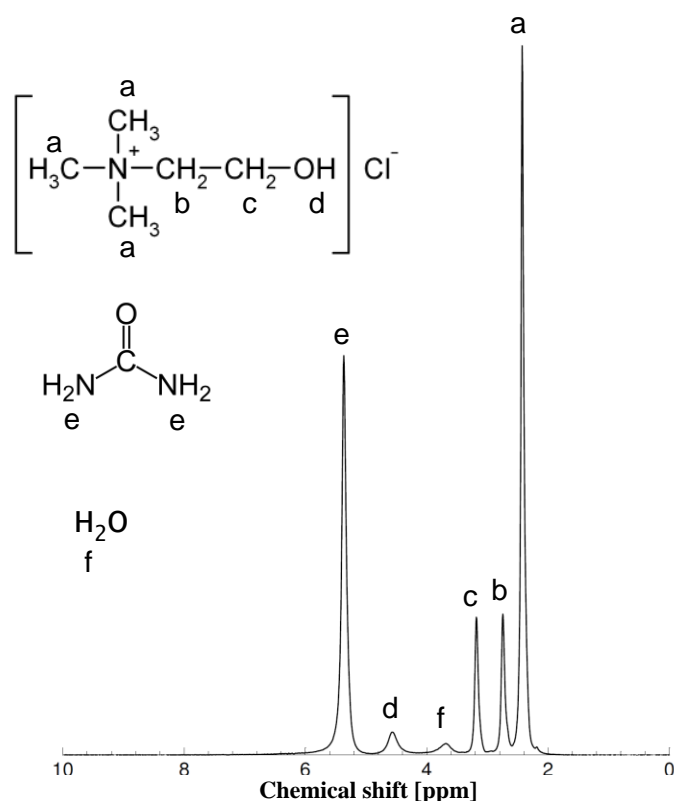
Figure 3. ^1\text{H} NMR spectrum of aqueous Reline at 1 wt% water content at 20 °C. The NMR peak positions are (in ppm): a = 2.43; b = 2.75; c = 3.18; d = 4.59; e = 5.38; f = 3.69. All resonances are quoted relative to the ^1\text{H} resonance of tetramethylsilane (TMS).
